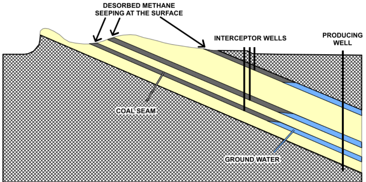
Figure 3: Cross section showing how gas interception system wells can be placed between CBM operations and the coal outcroppings where fugitive emissions occur in order to capture methane before it reaches the surface. Fugitive methane emitted at the surface can originate both from within the seam above the ground water level as well as from the main part of the CBM field below the ground water level
