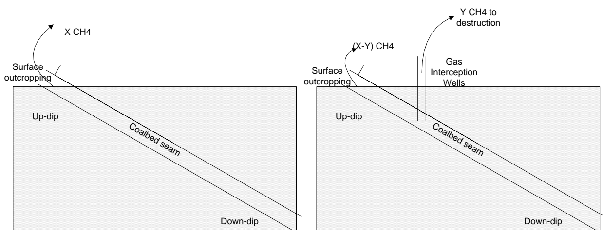
Figure 4: Schematic illustrating the change in fugitive emissions at the coal seam outcropping resulting from methane capture by the gas interception systems, in this case, vertical wells.
