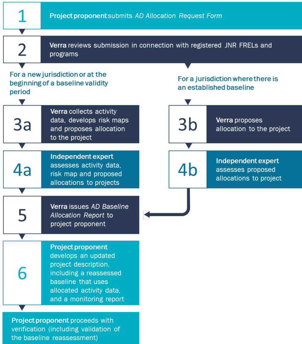
Figure 8: High-level baseline generation process for registered projects
