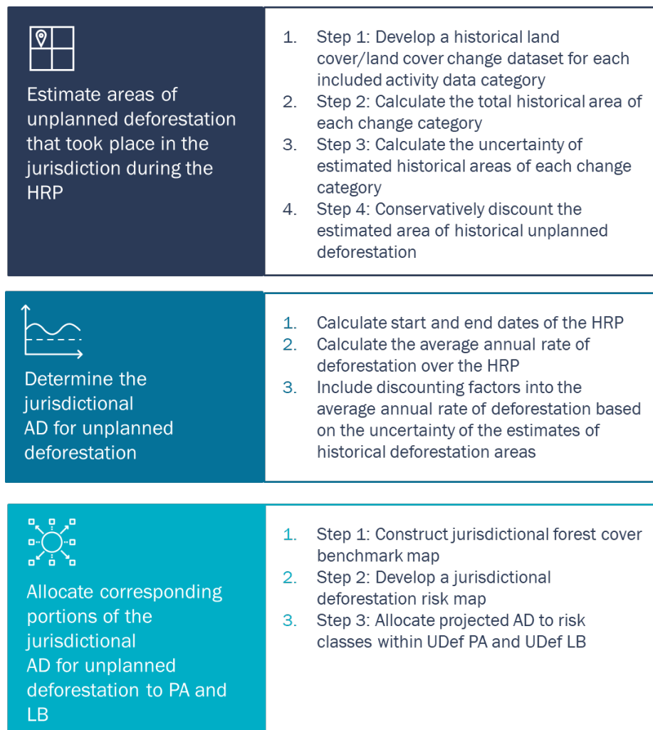
Figure 5: Allocation of jurisdictional deforestation AD to UDef PAs and UDef LBs
