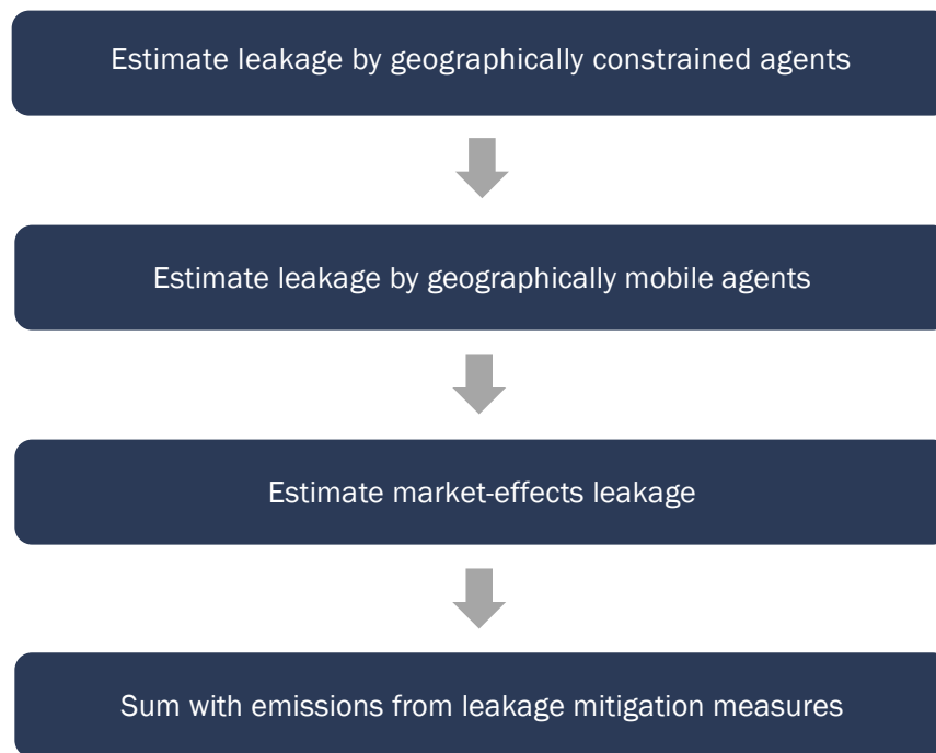
Figure 4: Leakage estimation steps
