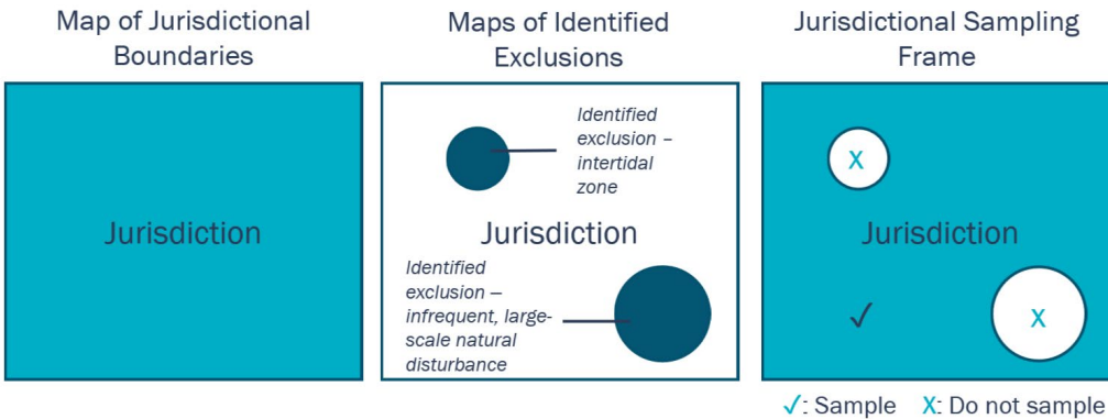
Figure 6: Conceptual illustration of the development of identified exclusion area maps and jurisdictional sampling frame
