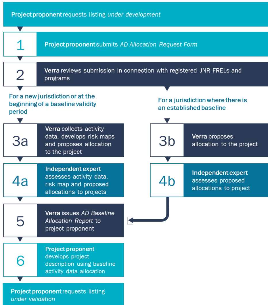
Figure 7: High-level baseline generation process for new projects
