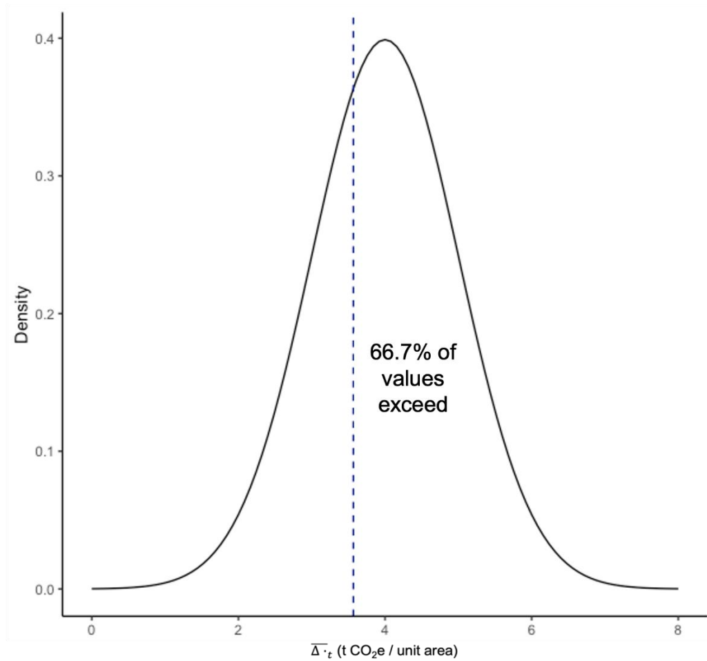
Figure 2. Probability of exceedance. The value for \overline{\Delta} \cdot t used in calculation of net reductions is determined by applying an uncertainty deduction based on the 33.3rd percentile of the estimated probability distribution of \overline{\Delta} \cdot t
