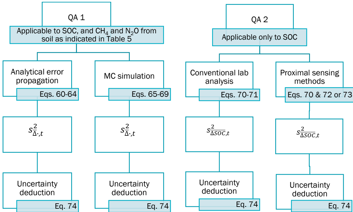
Figure 54: Equation map for calculating uncertainty deduction under Quantification Approaches 1 (for SOC, CH 4 and N 2 O) and 2 (for SOC) 59
