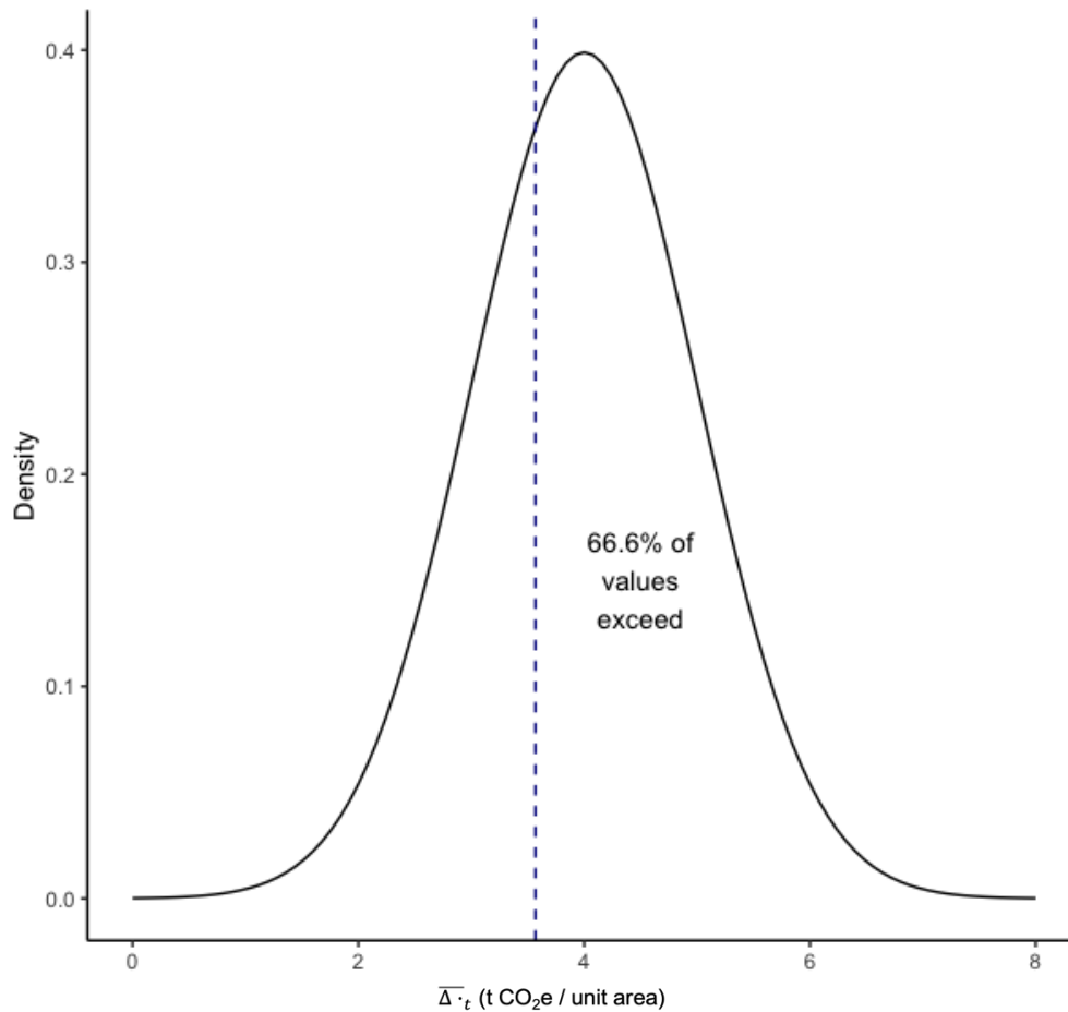
Figure 43: Probability of exceedance. The value for \bar{\Delta}_t used in calculation of VCUs issued is determined by applying an uncertainty deduction based on the 33.3rd percentile of the estimated probability distribution of \bar{\Delta}_t
