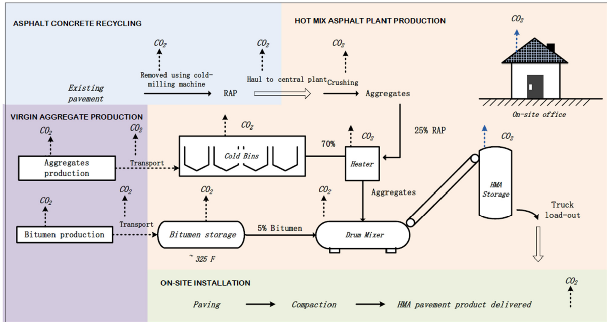
Figure 2: Diagram of HMA Production and Placement
