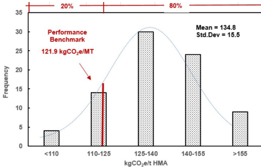
Figure A1: Illustration of Performance Benchmark for Hauling Distance less than 40 Miles
