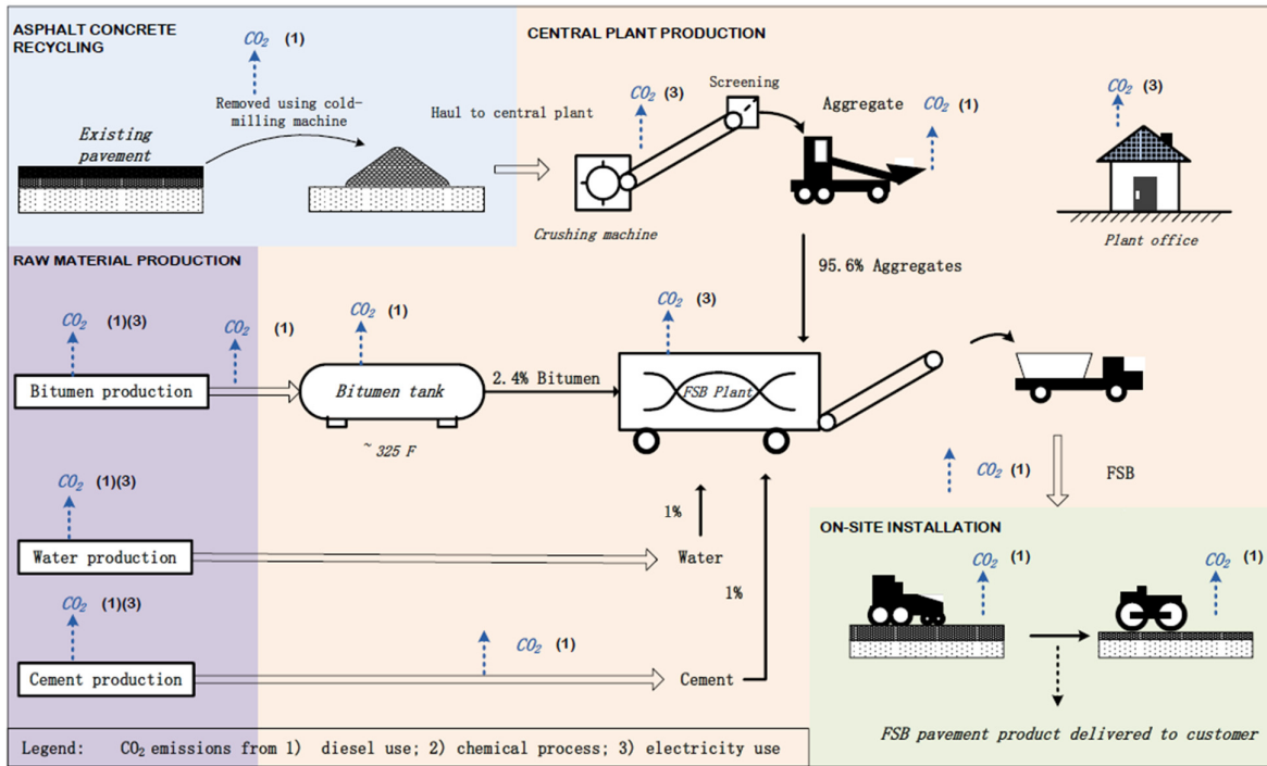
Figure 3: CCPR Project Activities and Associated GHG Sources
