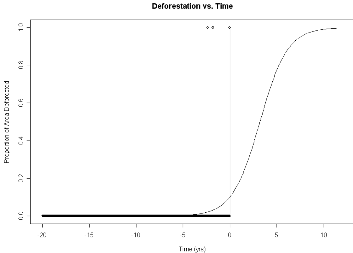
Figure 9: Graph of an example logistic function determined by \alpha , \beta and \theta . A graph of the estimated logistic function over time for the example reference area relative to the project state at time zero.
