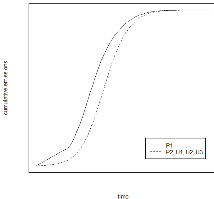
Figure 17: Graph of cumulative emissions from deforestation for the different baseline types
