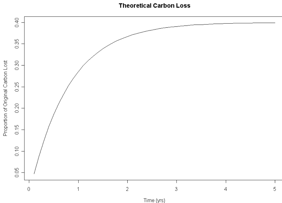
Figure 10: Graph of asymptotic soil carbon loss.
