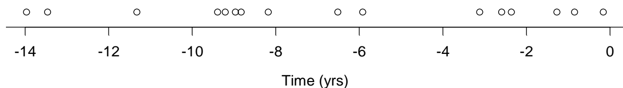
Figure 3: Line plot to demonstrate stationary of historical imagery.
