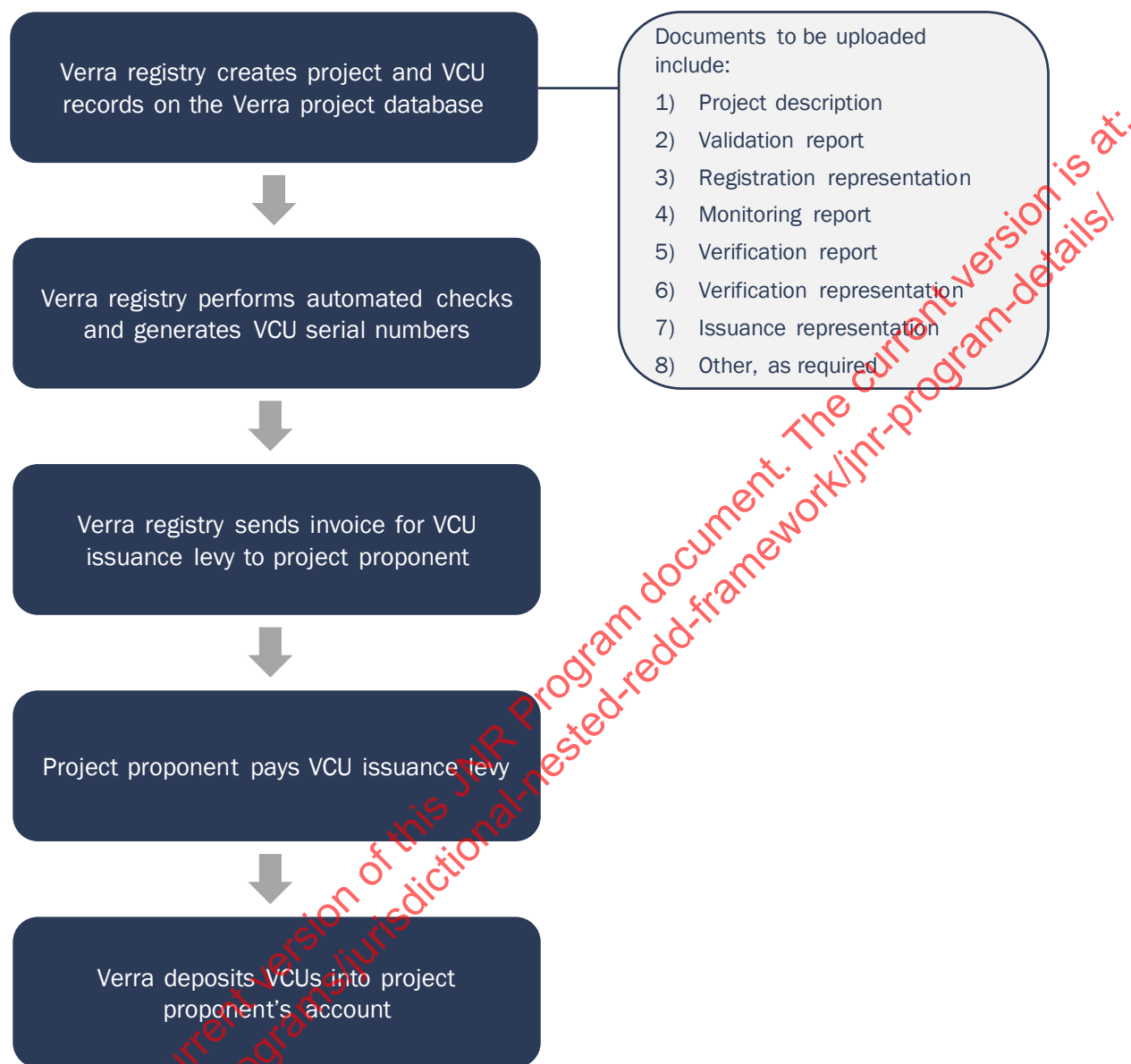
Diagram 4: Jurisdictional Element Registration and Initial Jurisdictional Program VCU Issuance
